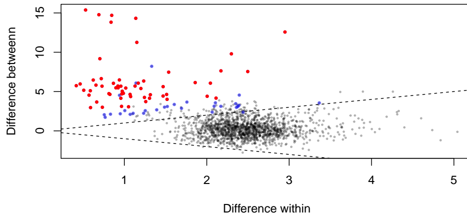
Figure 2: Differential abundance in the selex dataset using the Welch's t-test, Wilcoxon rank test, Kruskal-Wallace test or glm function. Features identified by all tests shown in red. Features identified by three or fewer tests are shown in blue dots. Non-significant features represent rare features if black and abundant features if grey dots.
